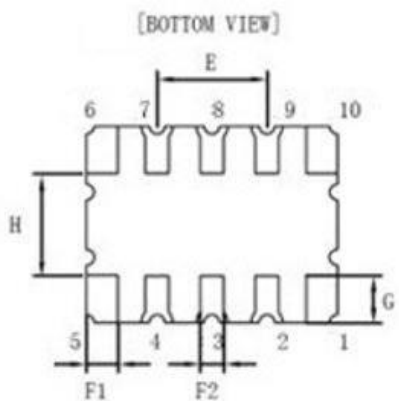
Figure 2. Dimension
