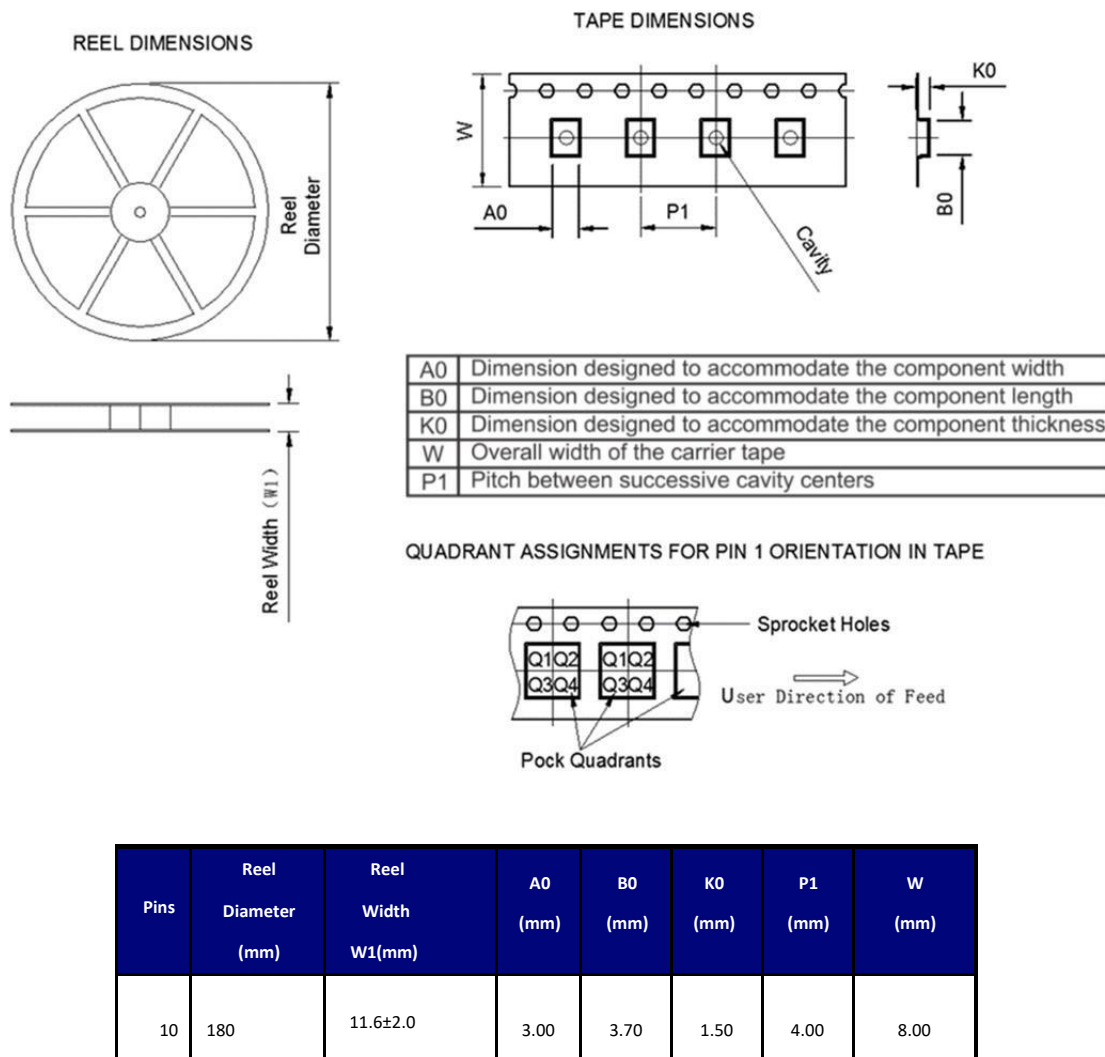
Figure 4. Package
