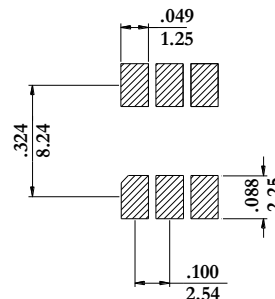
RECOMMENDED SOLDER PATTERN TOP VIEW
