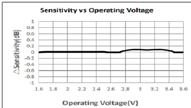
Sensitivity vs Operating Voltage
