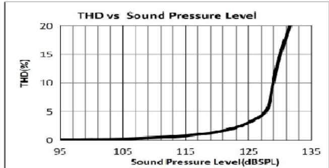
Typical THD vs Sound Pressure Level
