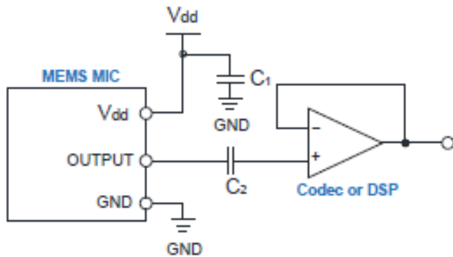
Single ended input interface circuit
