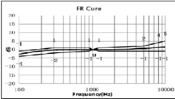
Frequency response curve normalized to 1kHz
