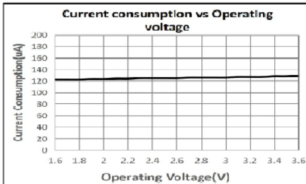
Current consumption vs Operating voltage
