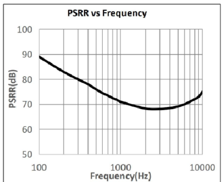
Typical PSRR cure
