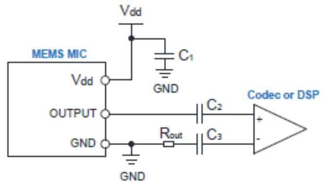
Differential input interface circuit
