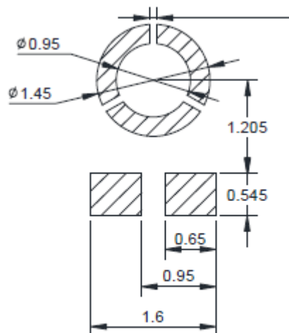
Solder Stencil Pattern
