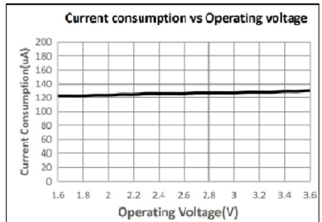
Current consumption vs Operating voltage
