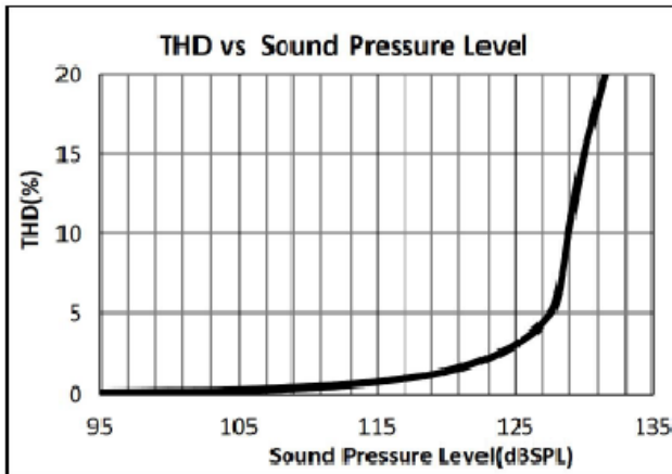
Typical THD vs Sound Pressure Level
