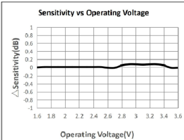
Sensitivity vs Operating Voltage
