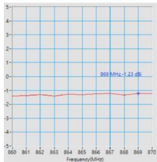
Maximum Peak Gain at 869 MHz : -1.23 dBi
